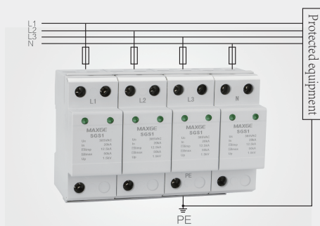
SGS1-T1/T2 Wiring diagram
